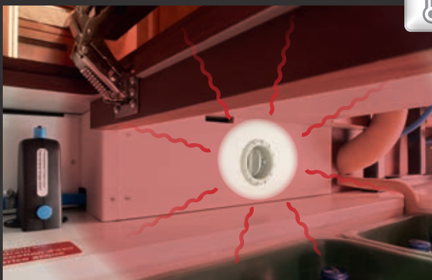
Truma Combi 6 warm air storage heating system with numerous warm air outlets throughout the double floor, the living area, the roller garage and the cold-sensitive door entrances.
